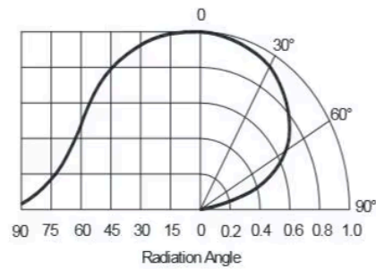
Typical Radiation Pattern 120°
